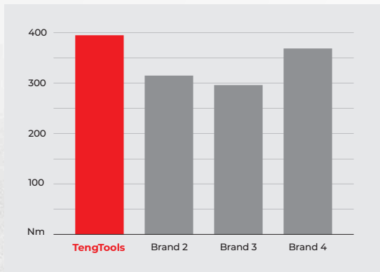
Adjustable wrench Comparison test. May 14, 2020. Torque breaking point (Nm). ISO 6787:2018.
